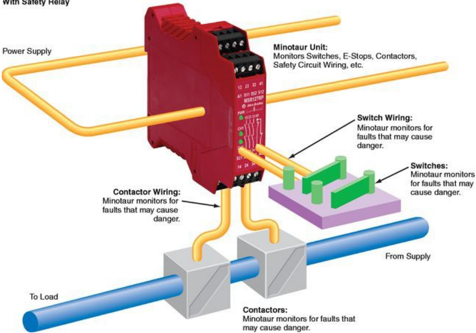
With Safety Relay
